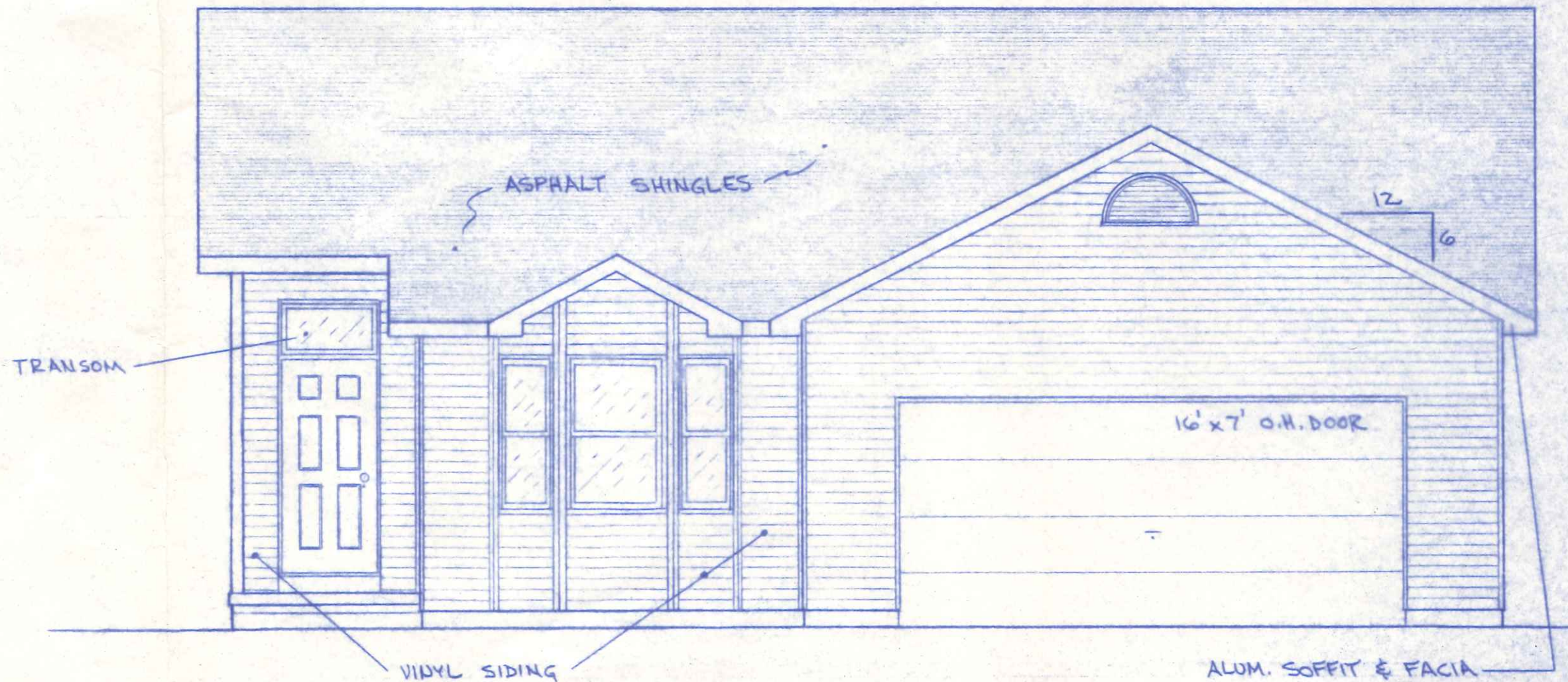
ALTERNATE FRONT ELEVATION
